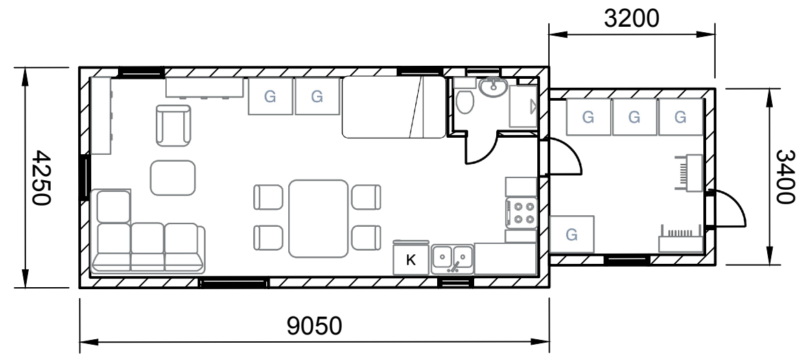
B-B (1:100)
